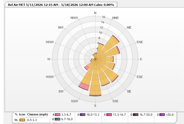
Figure 1: Meteorological Summaries
