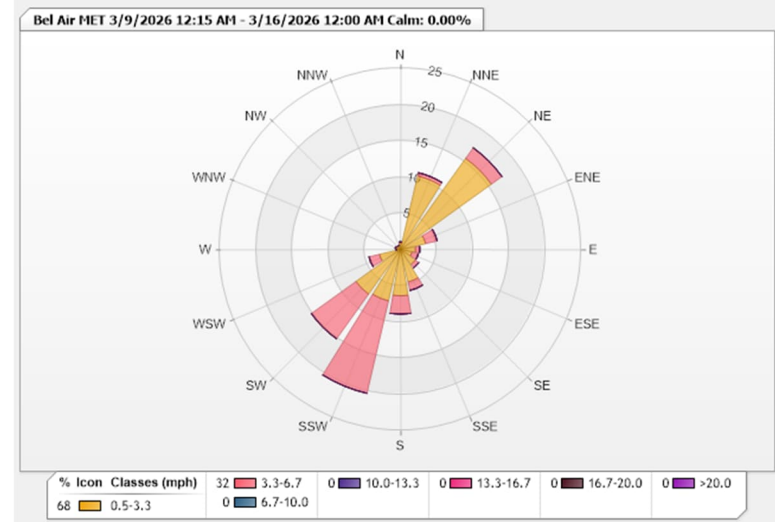
Figure 1: Meteorological Summaries
