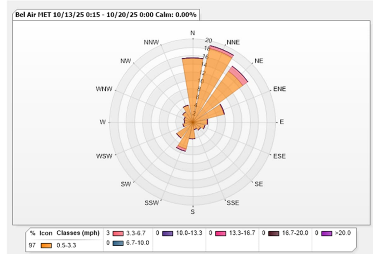
Figure 1: Meteorological Summaries
