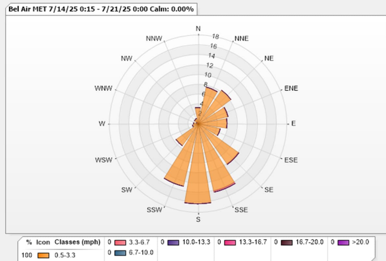
Figure 1: Meteorological Summaries
